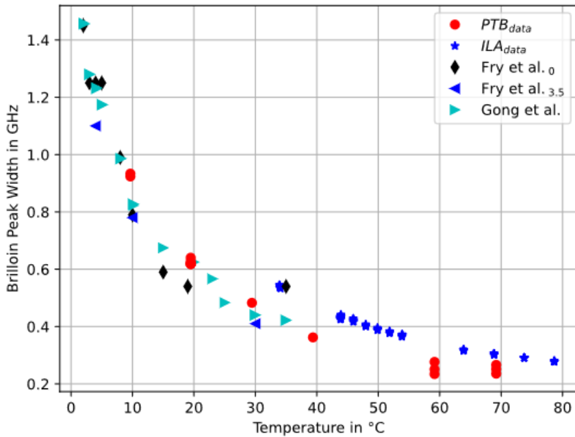
Figure 2: Brillouin peak width of water as a function of temperature, data either found in literature (Fry et al. 2002 for two different salinities, Gong et al. 2006) or obtained experimentally (labeled ILAdata and PTBdata)
