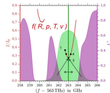
Fig.3: Frequency Scanning (FSM-FRS), iodine spectrum (pink), Rayleigh scattering spectrum (green) [Courtesy of Beuth Hochschule]
