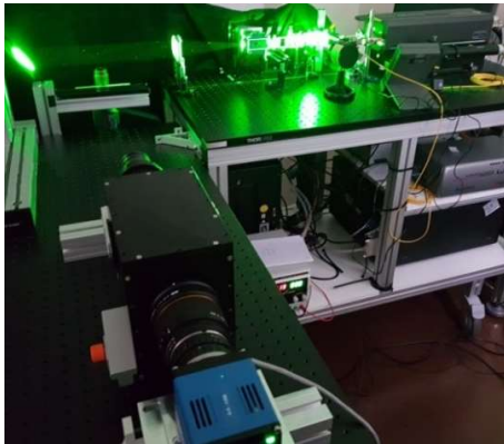
Fig.1: FRS Measurement of a heated free jet
