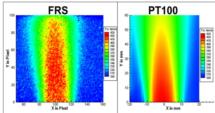
Fig.2: Comparison of the temperature distribution in a heated free jet with FRS and with a PT100 temperature probe
